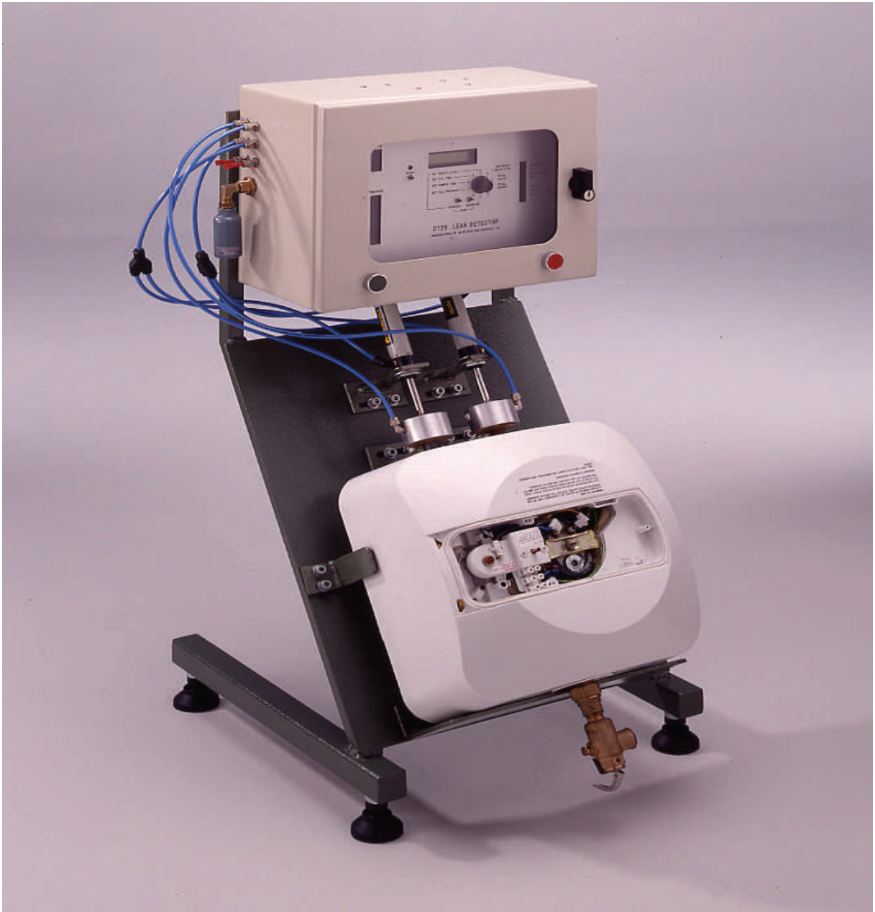
Bench Tester shown with water heater assembly. Unit sequences air flow to test check valves
